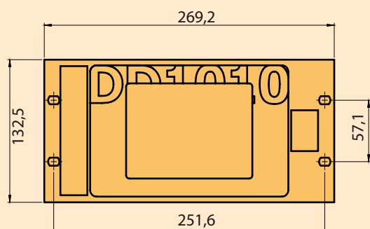
DD1010 rack version
